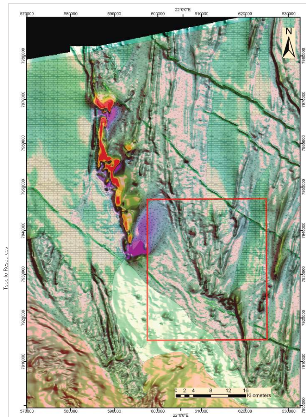
Appendix Figure 2 Structurally enhanced aeromagnetics data image overlain by geology (60% transparent). The outline shows the location of the current drilling site shown in text figure 10.
